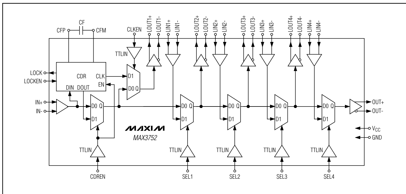
Figure 1. Functional Diagram
